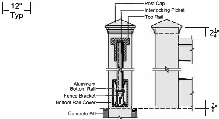
Post Profile: Cut View / Elevation View
