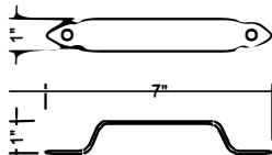
GATE HANDLE
