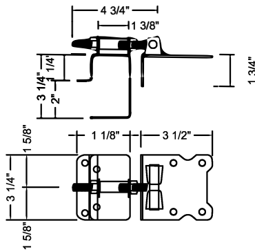
CUSTOM ADJUSTABLE HINGE
