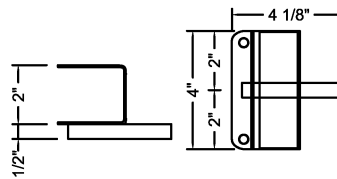
DOUBLE GATE STRIKER
