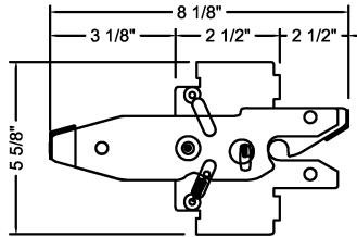
SINGLE GATE LATCH
