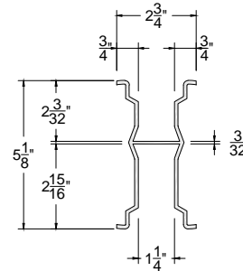
Aluminum Bottom Rail Profile
