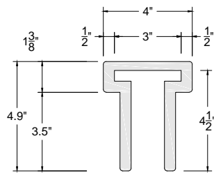
Top Rail Profile
